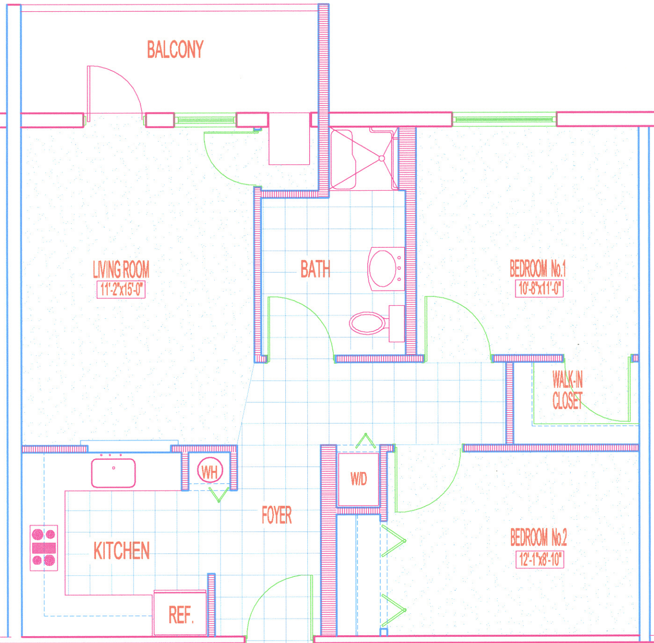
TYPE 'E' - 2BR UNIT FLOOR PLAN (750 SF)
